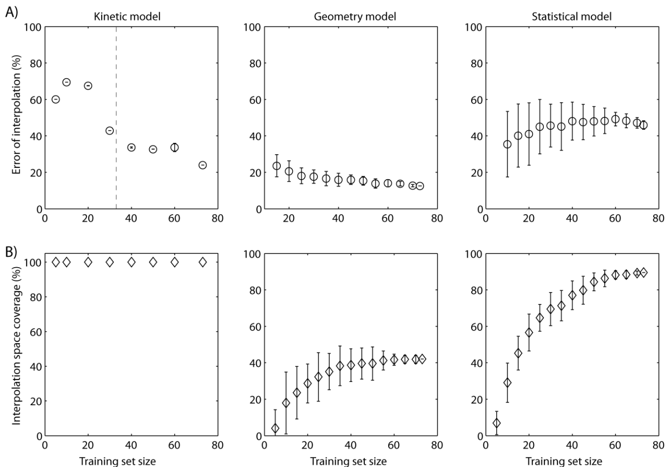
Supplementary Figure S10: Effect of training set size on model predictions. (A) Error of interpolation (B) percentage of the test set pathway variants that could be evaluated by the models. To have a reliable prediction from kinetic model, the training set size should be larger than the number of unknown parameters in the model (dashed line).
